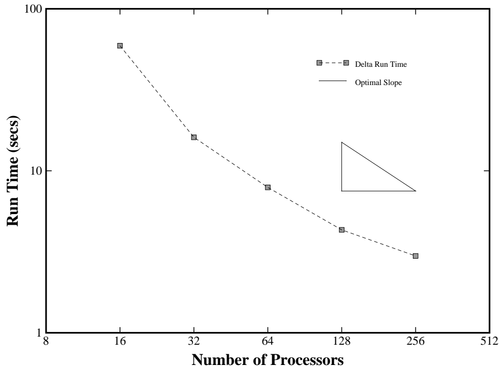
FIGURE 6. Scaling of the BDD algorithm
