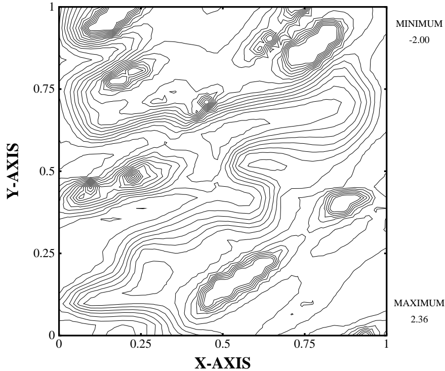
FIGURE 5. Coefficient of Test Problem III
