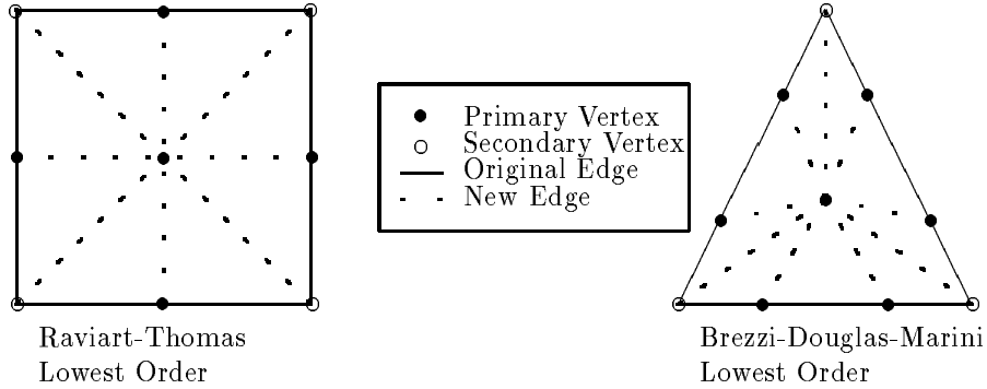
FIGURE 1. Examples of subtriangulations of two commonly used elements for all i, j = 1, \dots, k and all \lambda_i \in \Lambda_h(\partial\Omega_i) such that \int_{\partial\Omega_i \setminus \partial\Omega} \lambda_i \zeta_i ds = 0 , \forall \zeta_i \in \text{Ker}(s_i) , and s_i(\lambda_i, \zeta_i) = 0 , \forall \zeta_i \in Z_i . Then there exists a constant C not dependent on h, H or R , so that \kappa in Theorem 5.1 satisfies the bound
