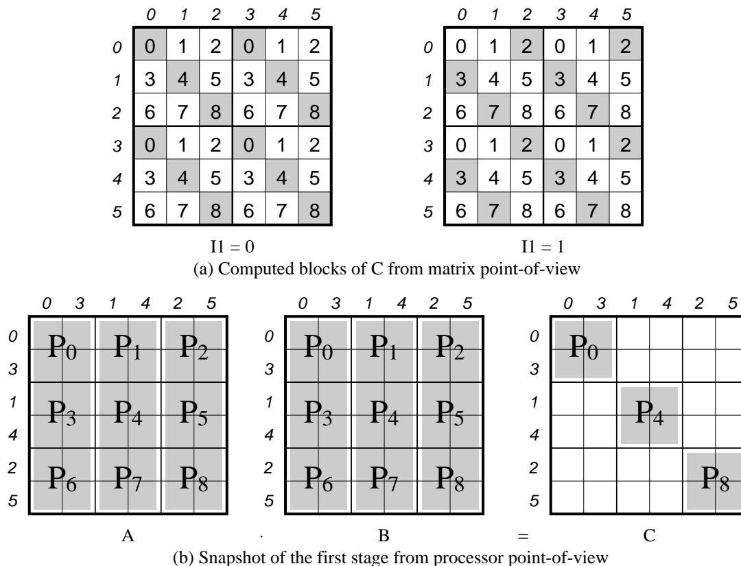
Figure 11: Snapshot of C = A^T \cdot B when P = Q = 3 and M_b = N_b = L_b = 6 . (a) From the matrix point-of-view, the computed blocks of the matrix C in the first two stages of the transposed matrix multiplication algorithm are shaded. (b) Snapshot of the first stage from the processor point-of-view. The shaded area of A and B represents blocks to be multiplied, and that of C denotes blocks computed from the multiplication. Only diagonal processors have results in the first stage. After each stage, A is shifted to the left.
