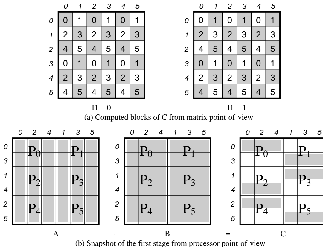
Figure 12: Snapshot of \mathbf{C} = \mathbf{A}^T \cdot \mathbf{B} when P = 3 , Q = 2 , and M_b = N_b = L_b = 6 . (a) From matrix point-of-view, the computed blocks of the matrix \mathbf{C} in the first two stages of the transposed matrix multiplication algorithm are shaded. (b) Snapshot of the first stage from processor point-of-view. If P and Q are relatively prime, the computed blocks of \mathbf{C} are scattered over all processors in each stage.
