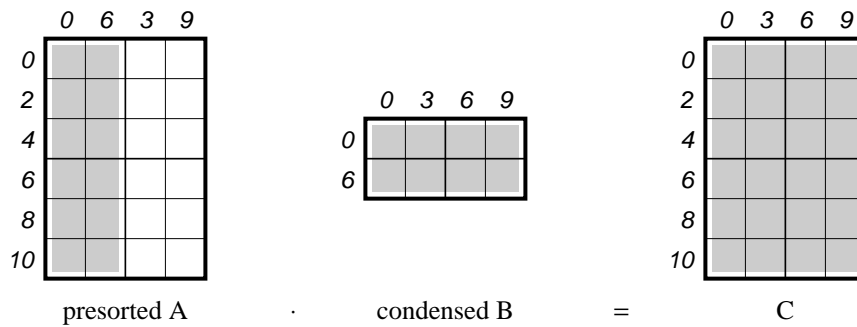
(b) computation in P_0 with presorted A
