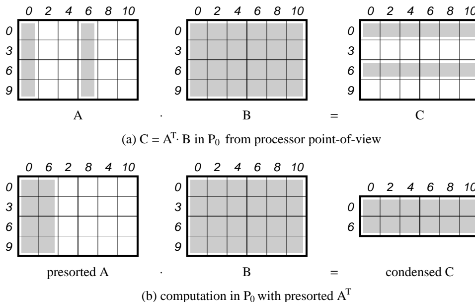
Figure 13: C = A^T \cdot B in P_0 from processor point-of-view, where P = 3 , Q = 2 and M_b = N_b = L_b = 12 . The shaded area of A and B represents blocks to be multiplied. And that of C stands for the result blocks to be placed after multiplication and summation processes over the column of the template.
